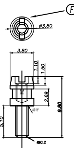
SECTION: B-B
